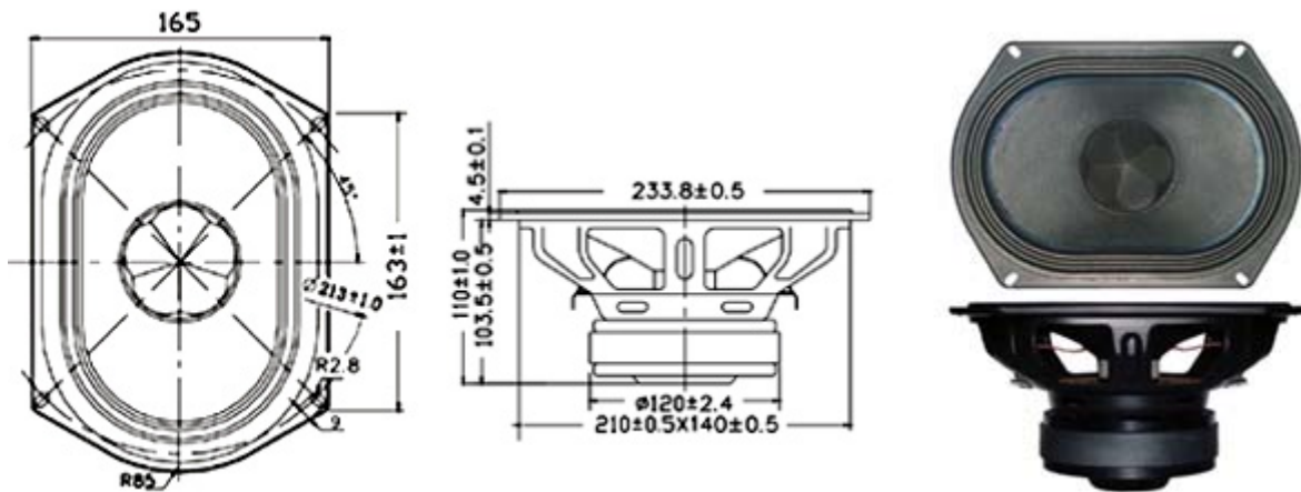
6*9" PAPER SUBWOOFER
