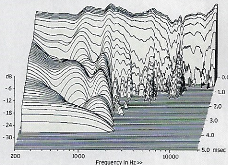
ABOVE: Resonances are coincident with peaks in the response, most obvious here at 800Hz and 1.4kHz
